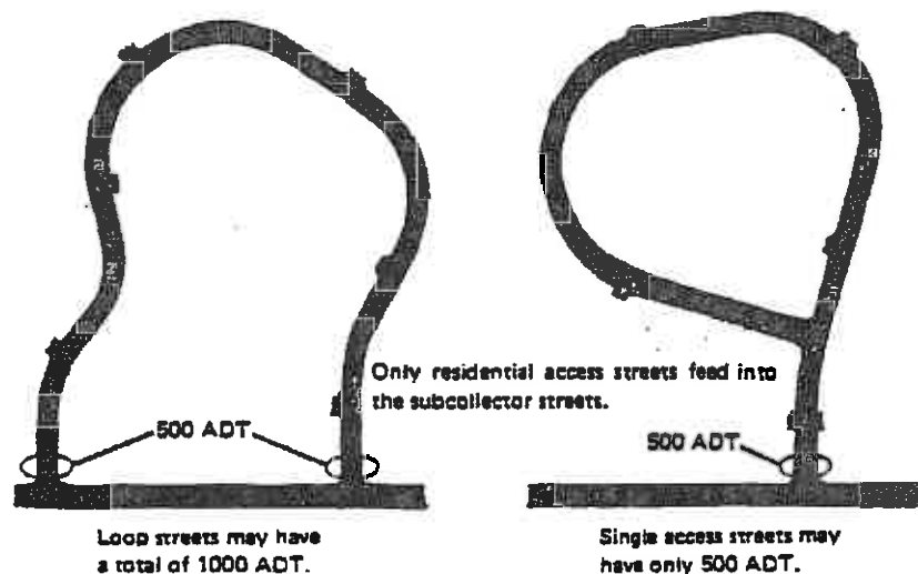
Service restrictions for residential subcollector streets.
