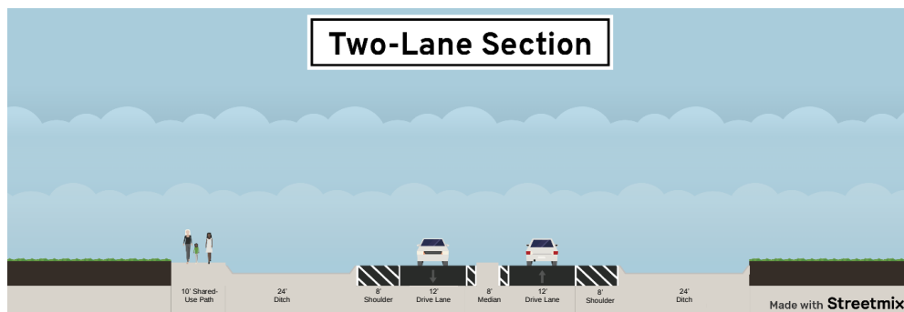
Figure A-1: Two-Lane Typical Section
