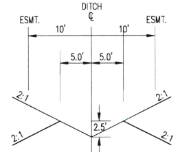
① TYPICAL 10' WIDE DRAINAGE DITCH ON PROPERTY SCALE: 1" = 10'
