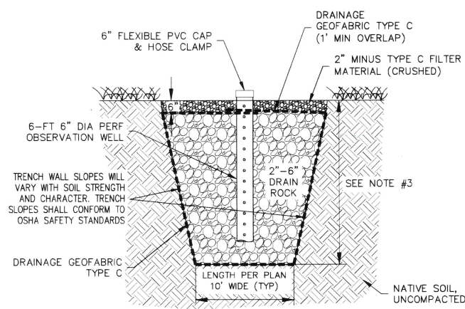
① TYPICAL 10' WIDE DRAINAGE DITCH ON PROPERTY SCALE: 1" = 10'
