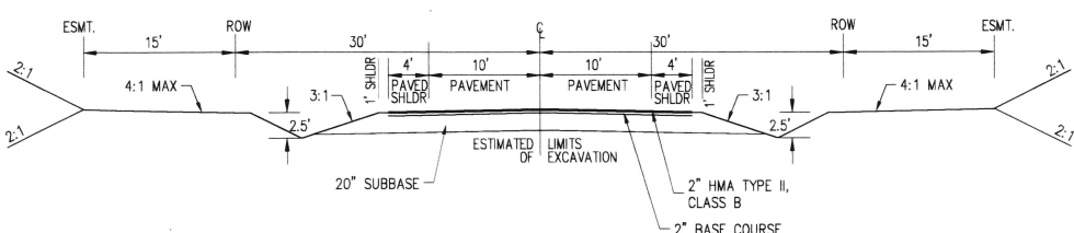
④ TYPICAL STREET SECTION - 28' WIDE PAVEMENT SCALE: 1" = 10'
