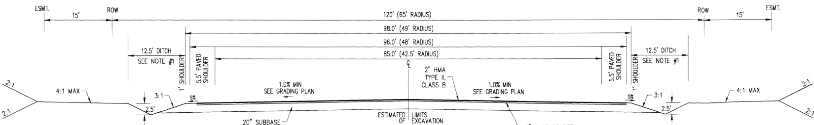
③ TYPICAL CUL-DE-SAC SECTION - 48.0' RADIUS SCALE: 1" = 10'
